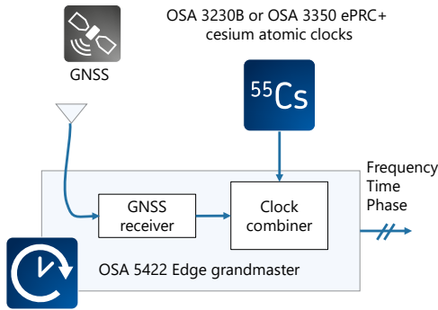
Compact ePRTC solution
