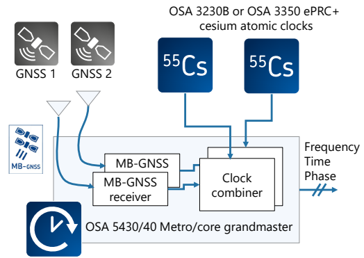
Redundant ePRTC solution
