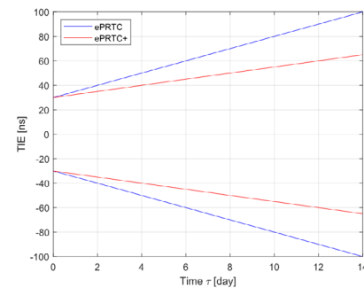
G.8272.1 ePRTC holdover versus OSA ePRTC+ holdover
